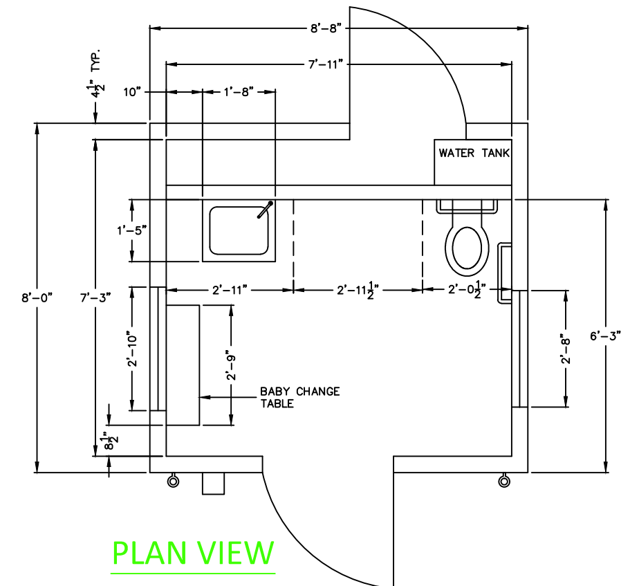
BACK COMPARTMENT
