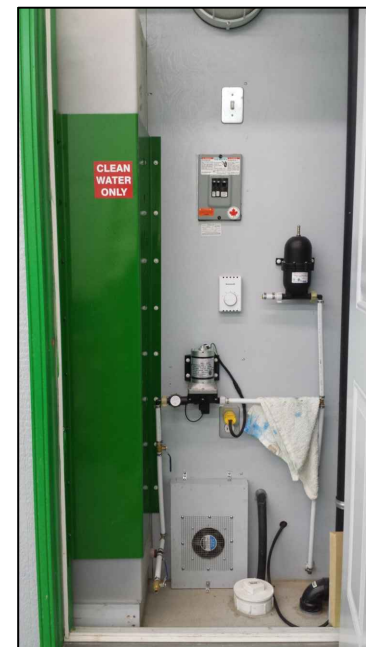
BACK COMPARTMENT
