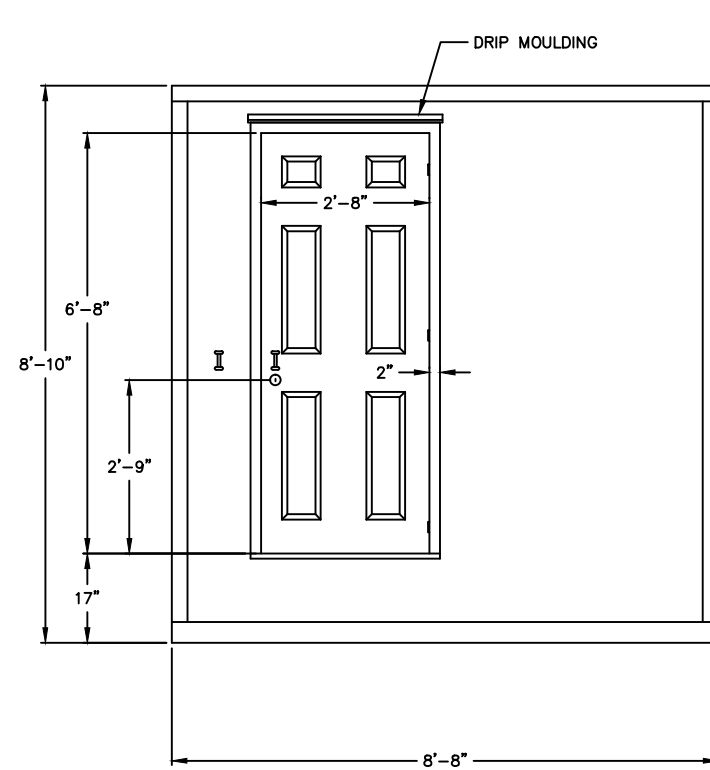
BACK ELEVATION
