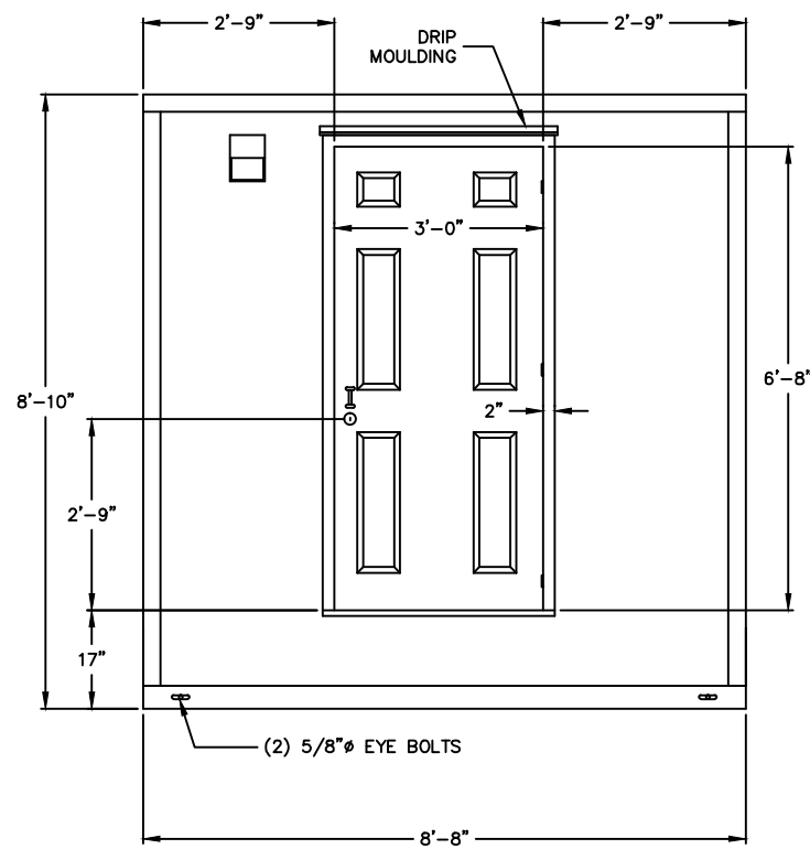
FRONT ELEVATION
